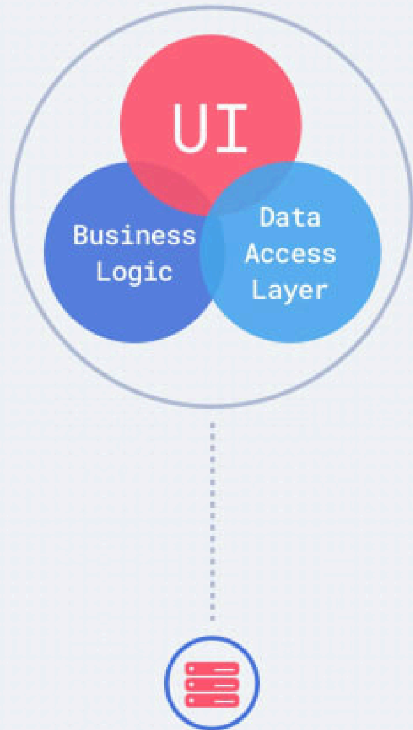
Monolithic Architecture
